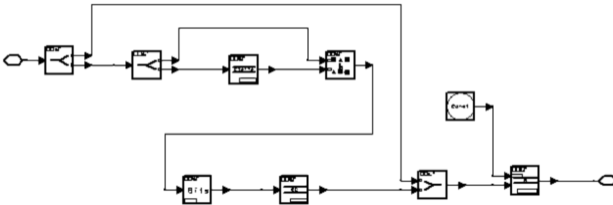
Schematic of Traffic Channel/Full-rate Speech (TCH/FS)
